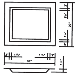
Recessed Sump Pan 29" x 33" x 14 GAGE Standard
