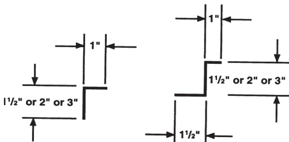
CELL CLOSURE
