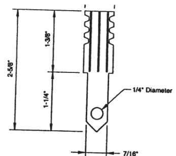
Piercing Hanger Tab Allowable Load 250 lb. when imbedded in concrete.
