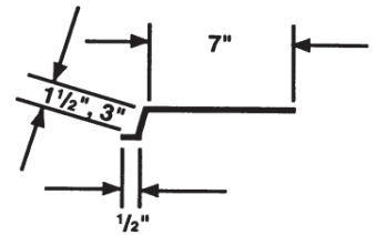
FILLER SHEET (20 GA.) 10'-0" LENGTHS GALVANIZED ONLY
