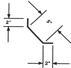
CANT STRIP (20 GA) 10'-0" LENGTHS GALVANIZED ONLY
