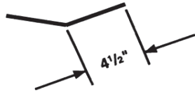
RIDGE OR VALLEY PLATE (20 GA.) 10'-0" LENGTHS GALVANIZED ONLY
